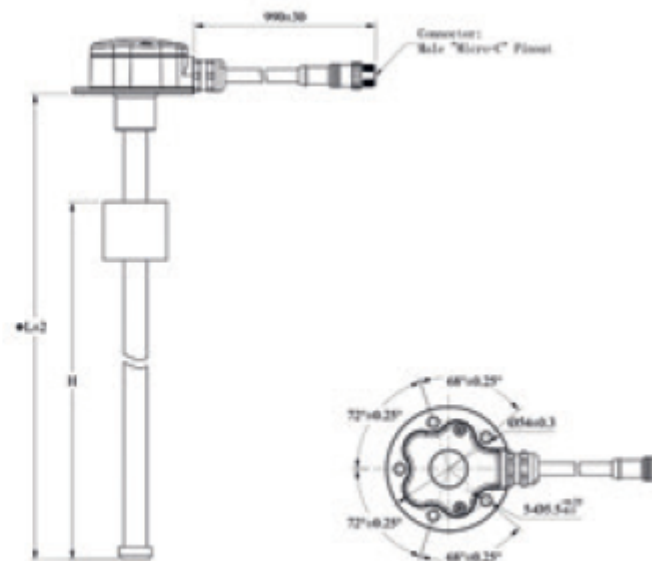
MOUNTING FLANGE SAE 5
